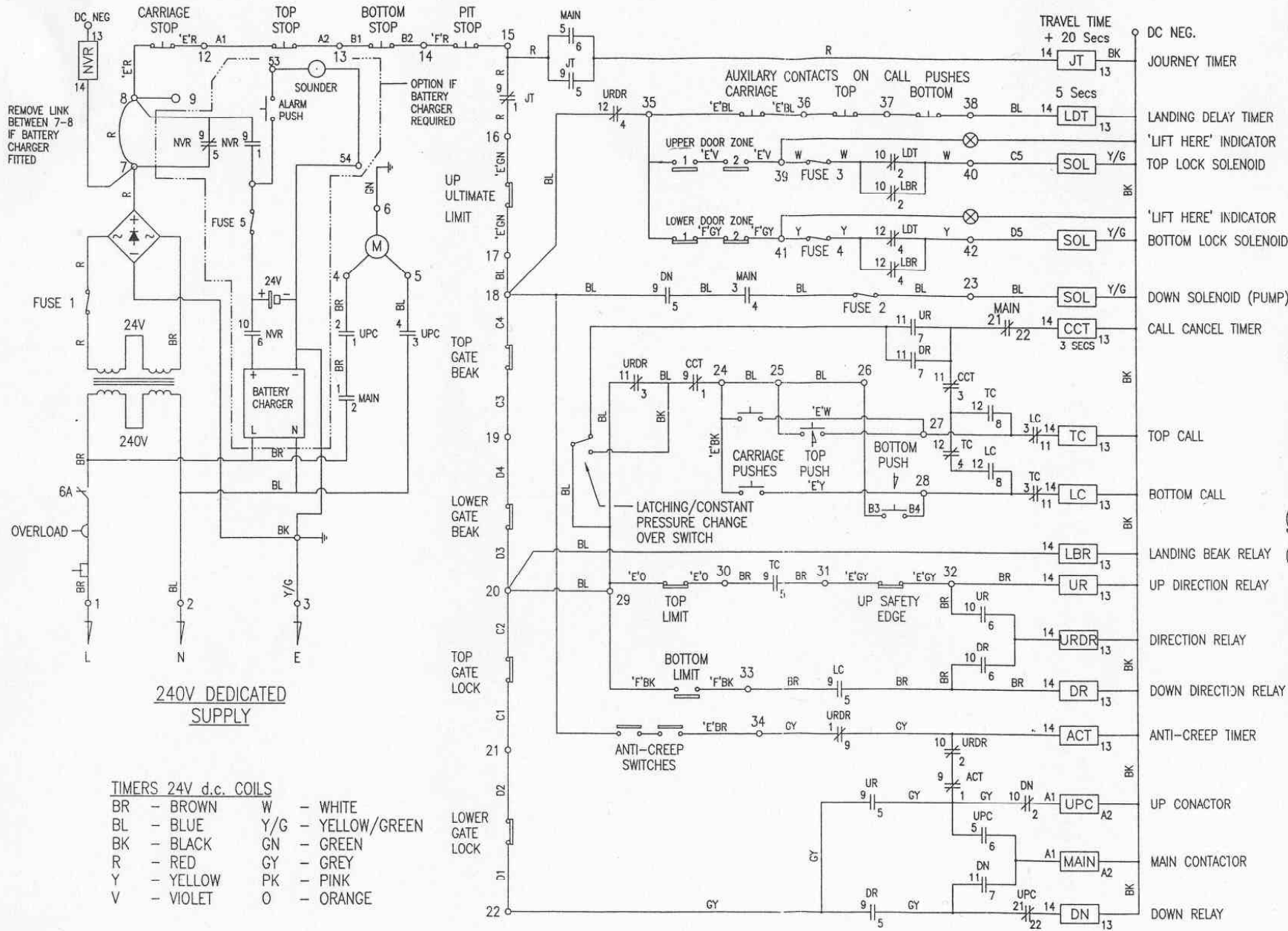
Wiring Schematic, Midlift PX iss 09.10.03 (standard swing doors, constant pressure controls) ref. 0230.8010 D
