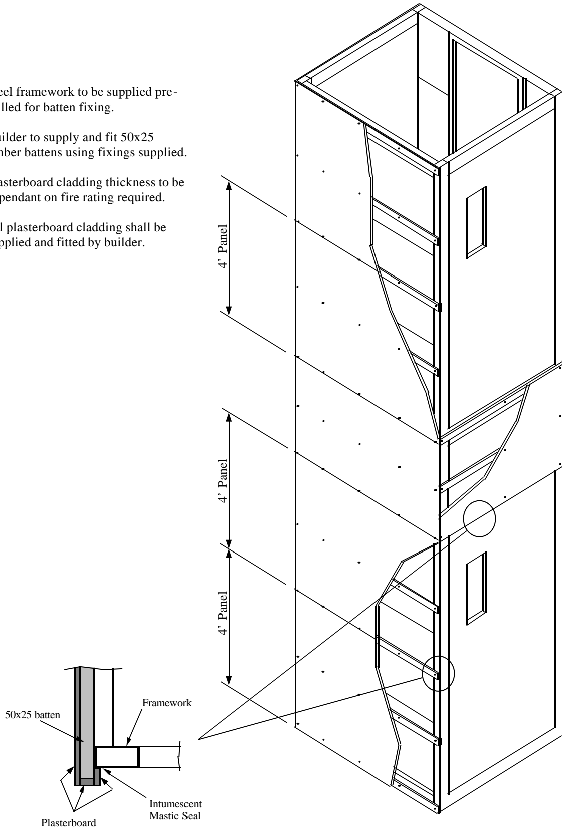
Enclosure with Plasterboard
