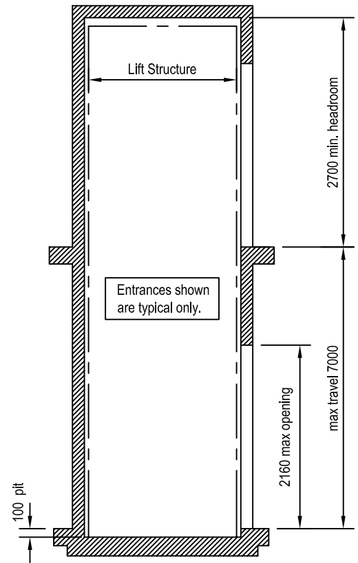
Lift Shaft Detail (optional)
