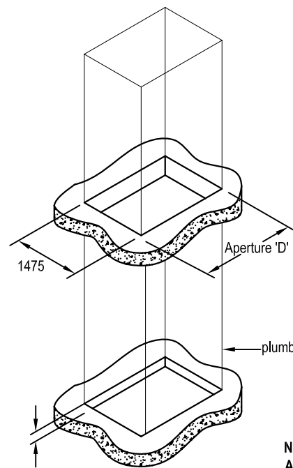
Pit & Aperture Detail (min. requirement)
