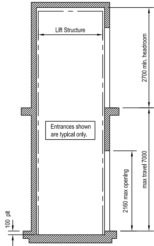
Lift Shaft Detail (optional)
