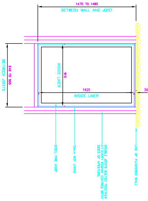
PLAN OF FLOOR APERTURE
