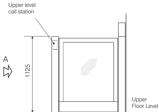
VIEW ON UPPER LANDING GATE Z
