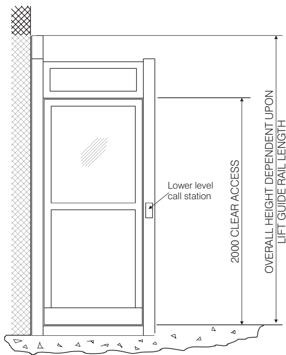
VIEW ON LOWER LANDING DOOR X
