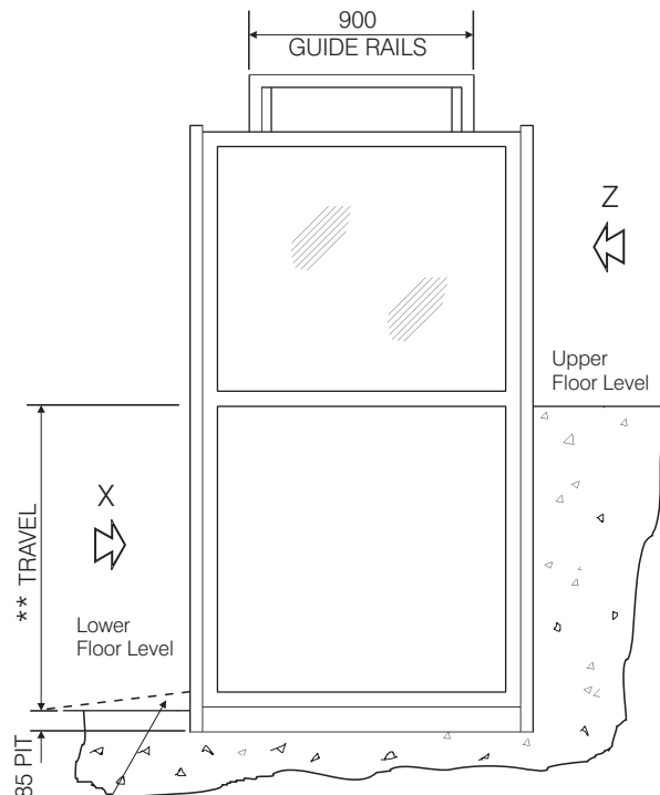
SIDE VIEW ON ARROW A
