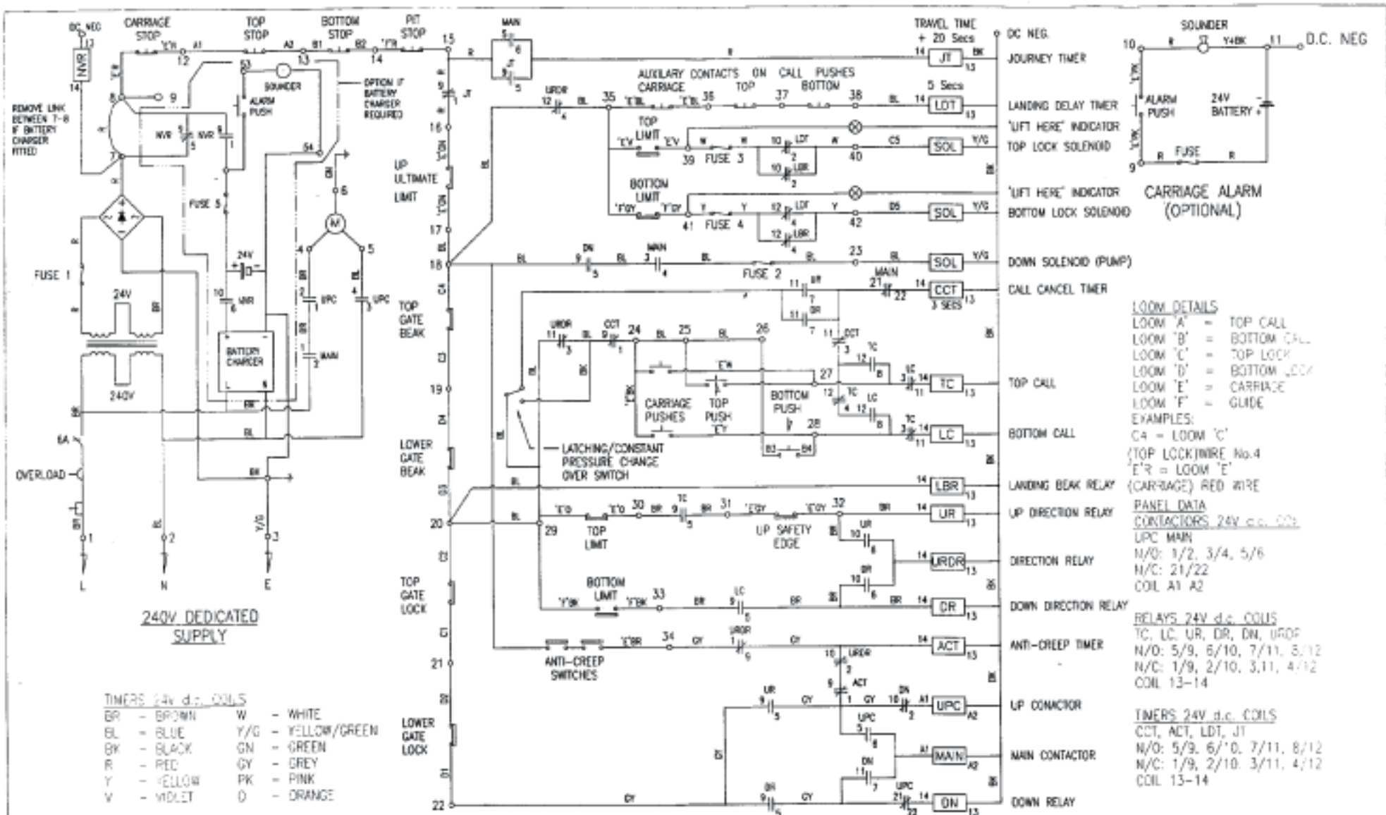
STANDARD WIRING DIAGRAM SWING DOORS WITH LATCHING/CONSTANT PRESSURE BUTTON CHANGE-OVER SWITCHING
